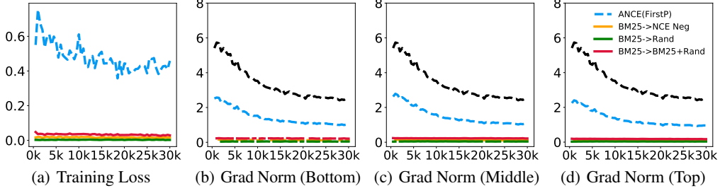
Figure 4: The loss and gradient norms during DR training (after BM25 warm up). The gradient norms are the per-layer average of the bottom (1-4), middle (5-8), and top (9-12) transformer layers. Black dotted lines are the grad norm of the last layer in ANCE (FirstP). The x-axes are training steps.
