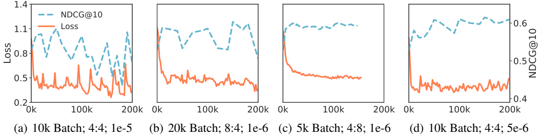
Figure 5: Training loss and testing NDCG of ANCE (FirstP) on documents. The sub captions list the ANN index refreshing rate (e.g., per 10k Batch), Trainer:Inferencer GPU allocation (e.g., 4:4), and learning rate (e.g., 1e-5). The x-axes are the training steps.
